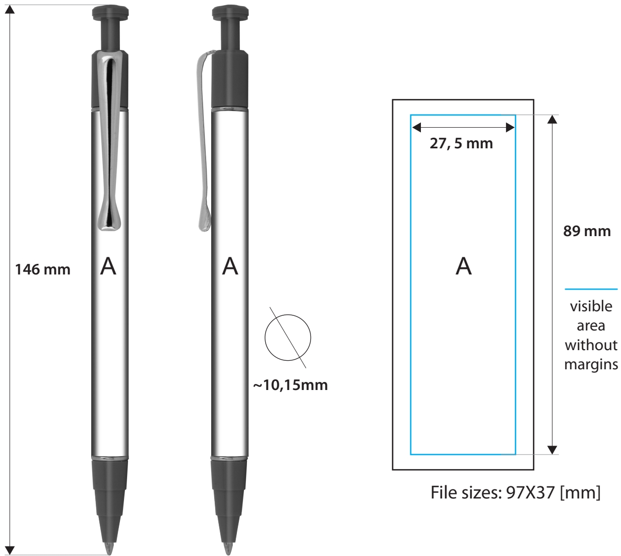
FRONT & LAT. VIEW - SCALE 1:1
